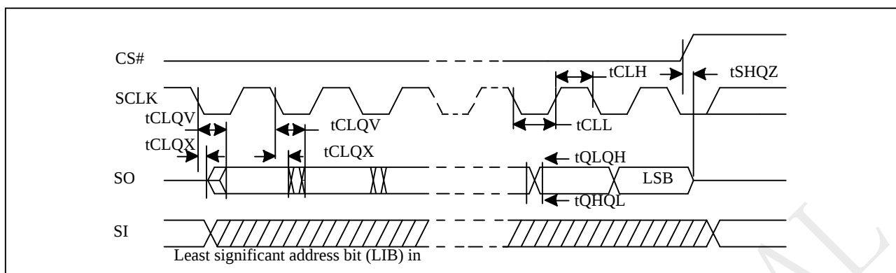
Figure 5-5 Output Timing
